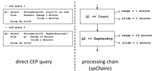
Fig. 4. Direct CEP query mapped on processing blocks
