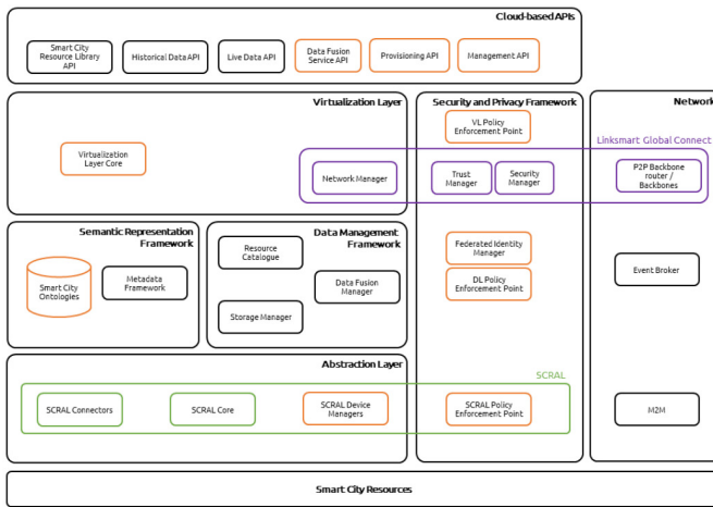
Fig. 1. The ALMANAC platform architecture
